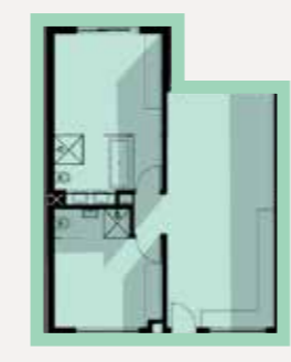
Type A(m) 2 Bedroom Unit
